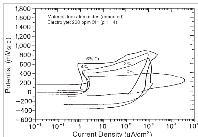
FIGURE 3. Cyclic anodic polarization curves of annealed (1 h at 859°C plus 7 days at 500°C) iron aluminides in aerated 200 ppm Cl - (pH = 4).
