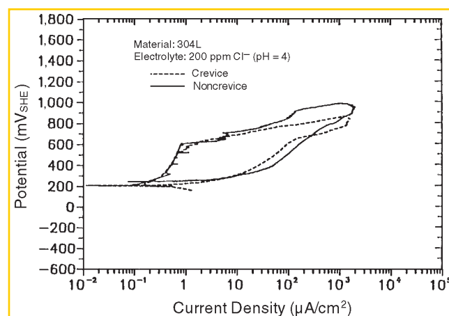
FIGURE 18. Comparison of cyclic anodic polarization curves of type 304L SS under crevice and noncrevice conditions in aerated 200 ppm \text{Cl}^- (pH = 4).
