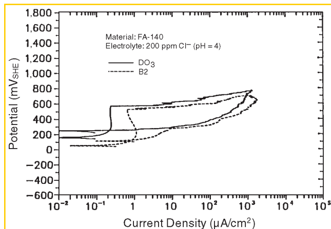
FIGURE 11. Effect of structure on the cyclic anodic polarization behavior in aerated 200 ppm \text{Cl}^- ( \text{pH} = 4 )
