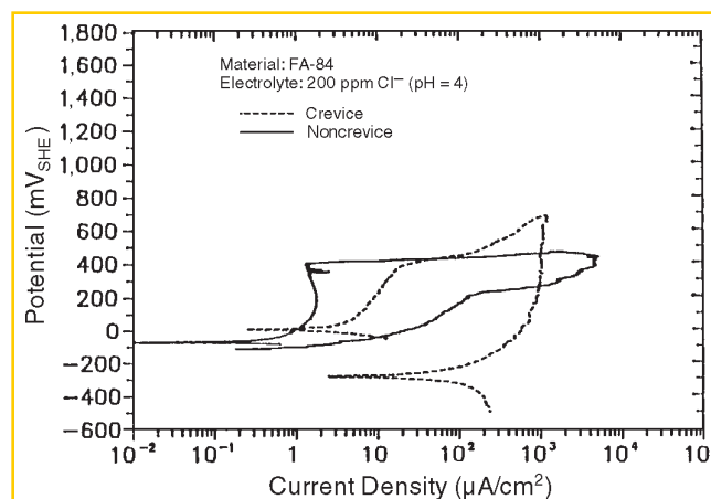
FIGURE 16. Comparison of cyclic anodic polarization curves of FA-84 (Fe-28% Al-2% Cr-0.05% boron [B]) under crevice and noncrevice conditions in aerated 200 ppm \text{Cl}^- (pH = 4).
