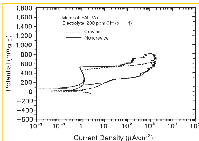
FIGURE 17. Comparison of cyclic anodic polarization curves of FAL-Mo (Fe-28%Al-5%Cr-1%Mo-0.04%B-0.08% zirconium [Zr]) under crevice and noncrevice conditions in aerated 200 ppm \text{Cl}^- (pH = 4).
